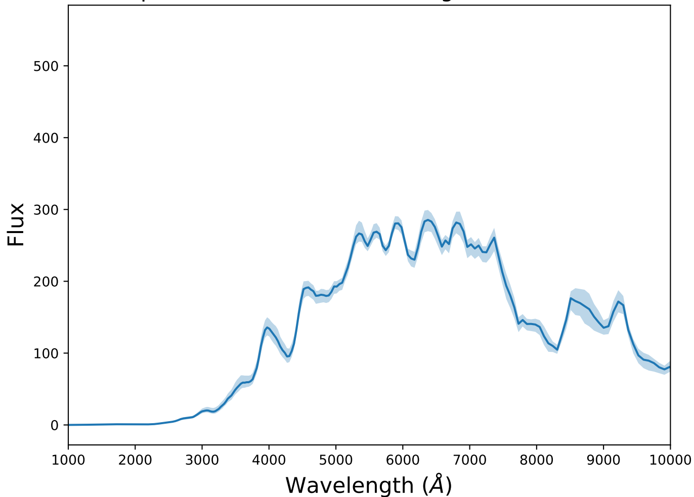
Spectrum 1 for transient 91bg-like at z=0.42
